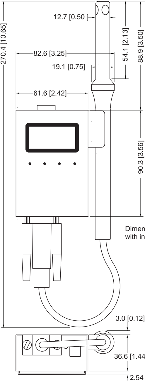
Figure 2.1 Dimensions
