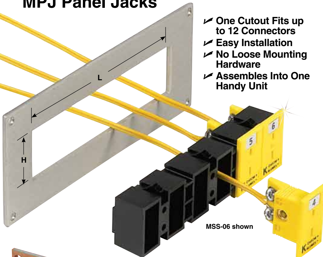
Miniature connectors
