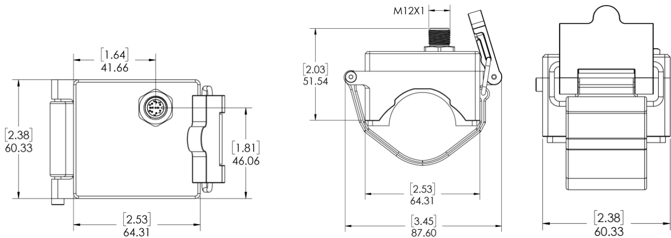
Figure 1: HANI™ Mechanical Dimensions in Inches
