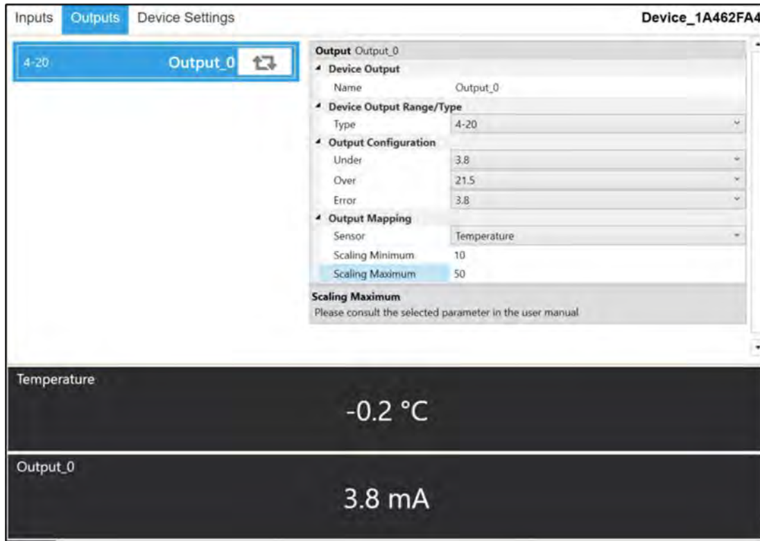
Figure 18: SYNC Configuration Software – 4-20 mA Output Sensor Mapping
