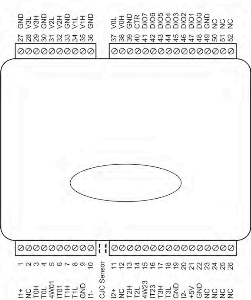
Figure 2. OM-USB-TEMP-AI screw terminal pin numbers
