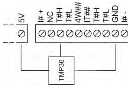
Figure 10. Semiconductor sensor measurement configuration
